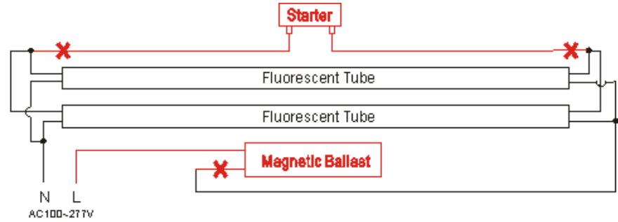
A Magnetic/Inductive Ballast w/ Starter
