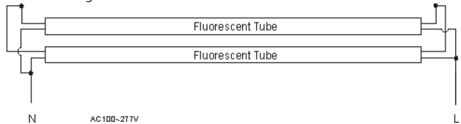
A Magnetic/Inductive Ballast w/ Starter
